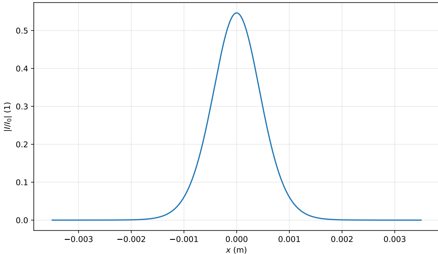
Intensity profile I(x, y = 0, z = 2.707m)/I_0 , P_{in}=0.4P_{cr} , artificial time
